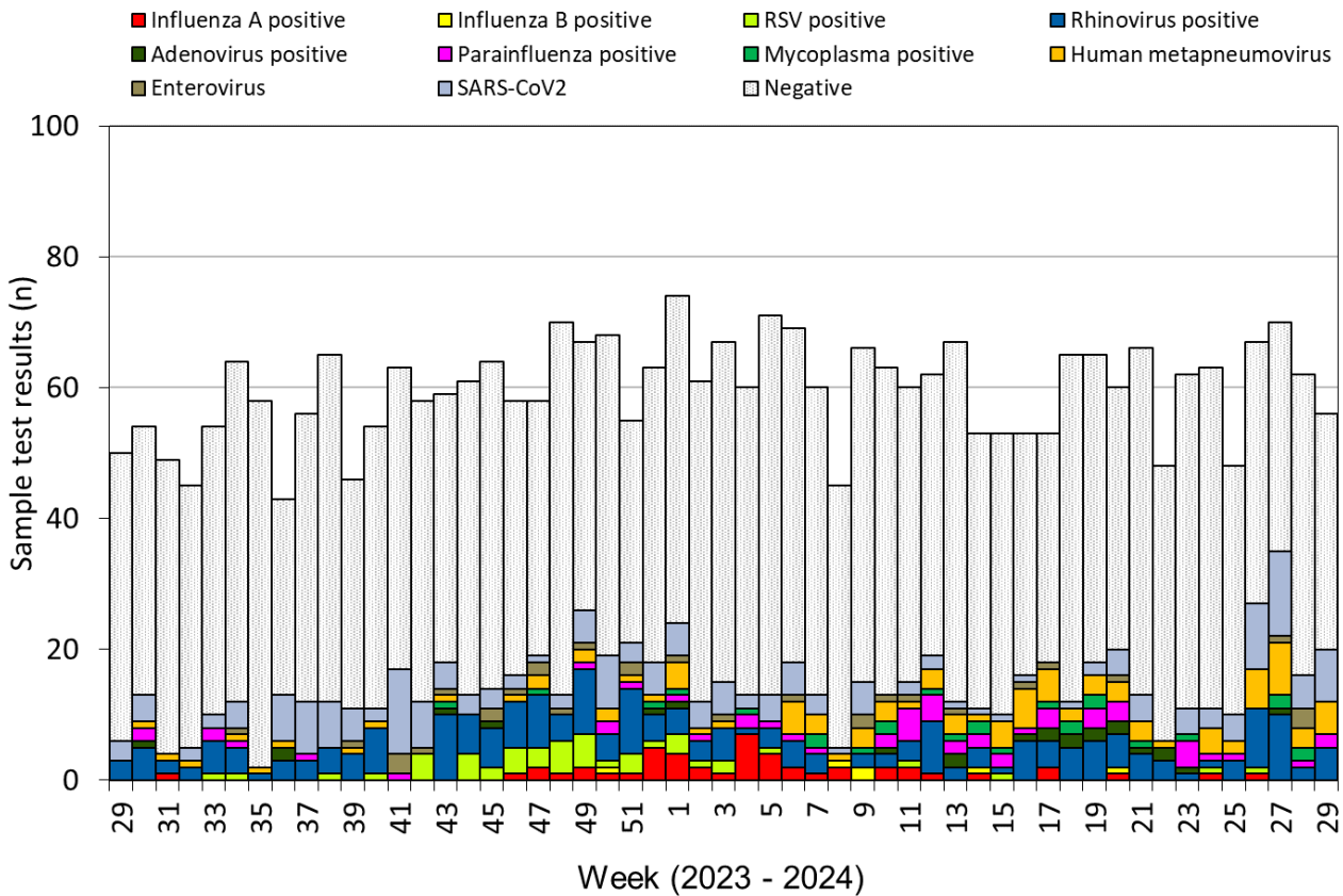
Figure 8. Specimens submitted for virological testing for ICU patients, by week of sample collection, Week 29 2023 to Week 29 2024.
