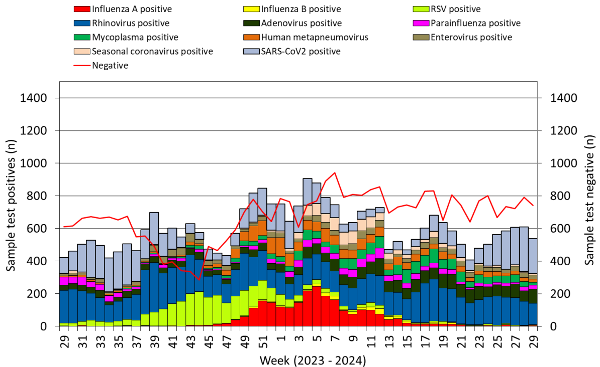
Figure 5. Specimens submitted for virological testing for hospital patients and non-sentinel GPs as of 14/07/2024 by week of sample collection, Week 29 2023 to Week 29 2024.
