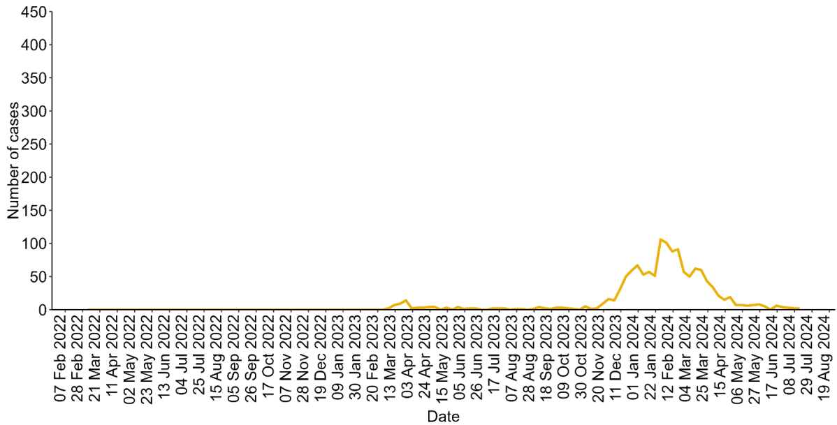
Figure 10. Seven day rolling sum of cases hospitalised in Wales within 28 days of an influenza positive test result in the community (or up to 2 days post-admission), as of 14/07/2024 (latest data available).
