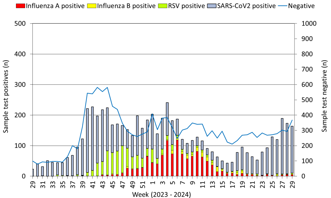
Figure 7. Specimens from hospital patients submitted for RSV, Influenza and SARS-CoV2 testing only, as of 21/07/2024 by week of sample collection, Week 29 2023 to Week 29 2024.
