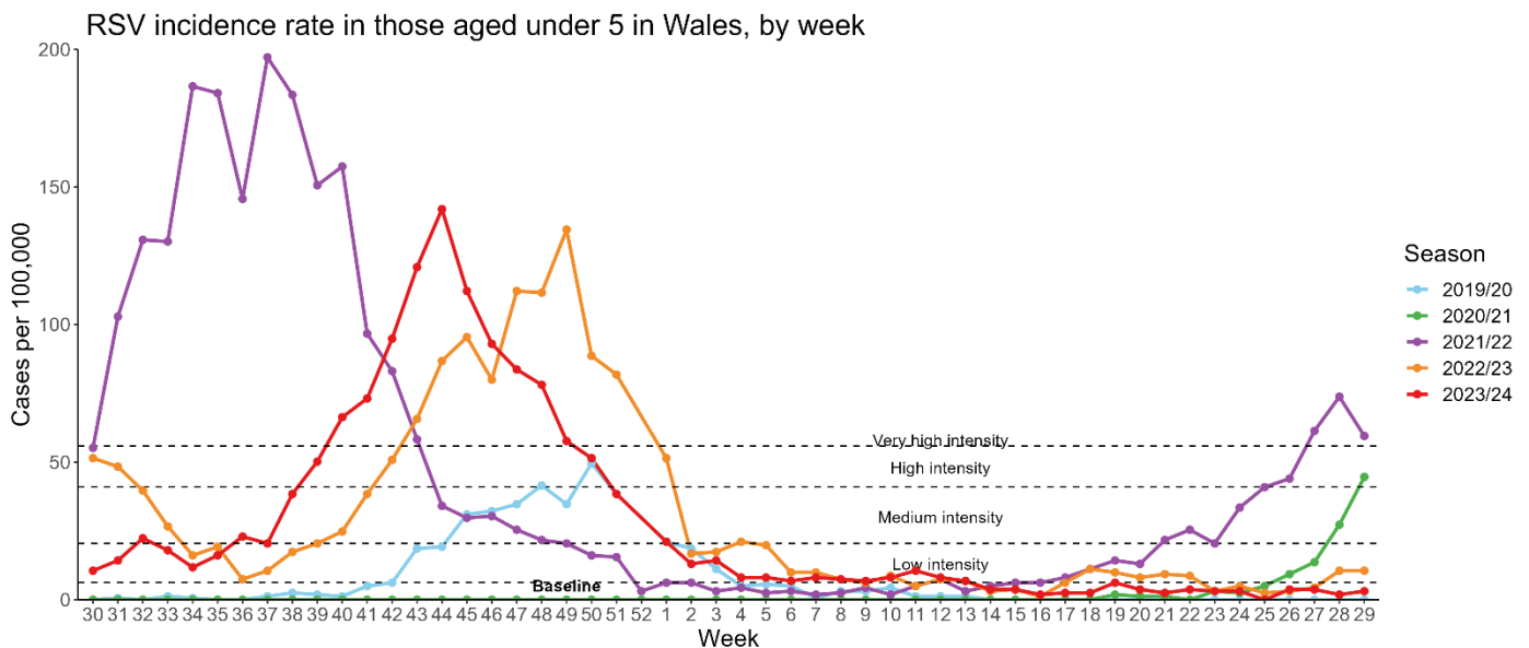
Figure 9. RSV incidence rate per 100,000 population aged under five years, week 30 2019 to Week 29 2024.
