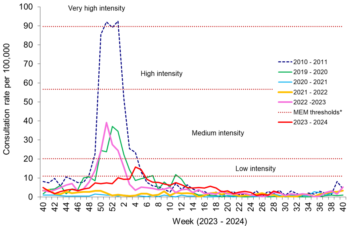
Figure 1. Clinical consultation rate for ILI per 100,000 practice population in Welsh sentinel practices (as of 21/07/2024)
