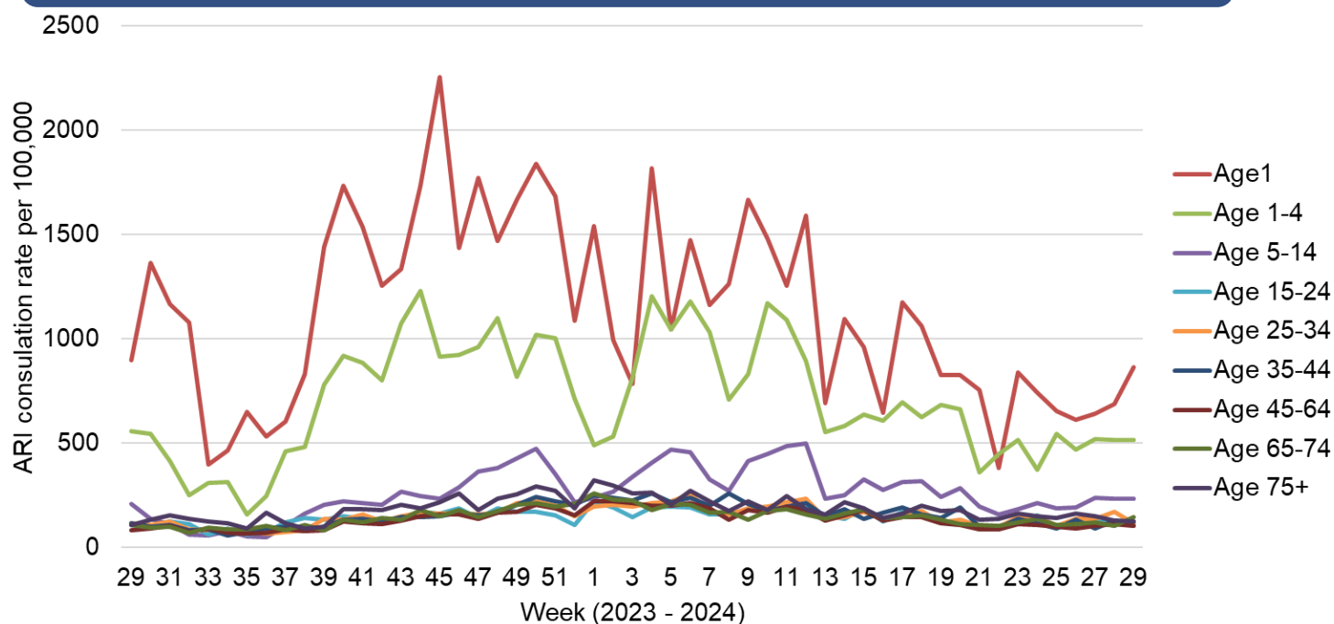
Figure 3. Age-specific consultations (per 100,000) for ARI in Welsh sentinel practices, Week 29 2023 – Week 29 2024.
